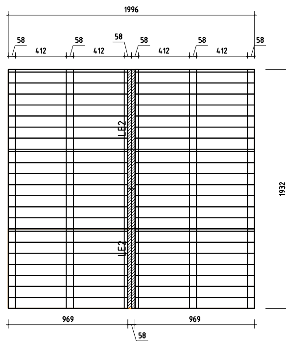
FUSSBODENPLAN - FLOOR PLAN
